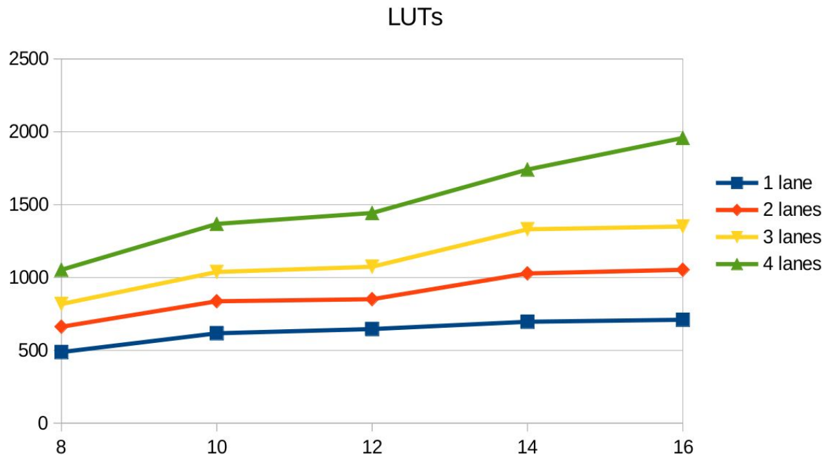
Figure 4 Tx: Resource utilization as a function of data width and number of lanes
