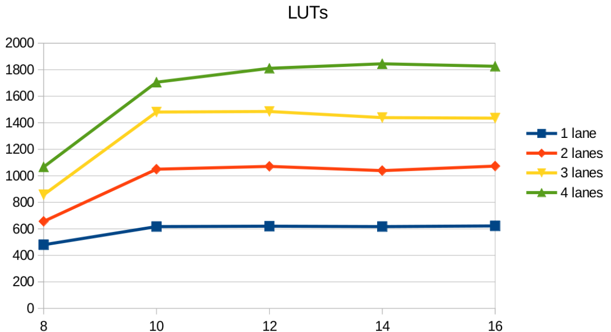
Figure 3 Rx: Resource utilization as a function of data width and number of lanes
